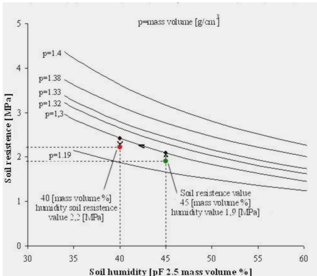
Figure 1. The method of converting the soil resistance values at various humidity values into identical humidity values.
