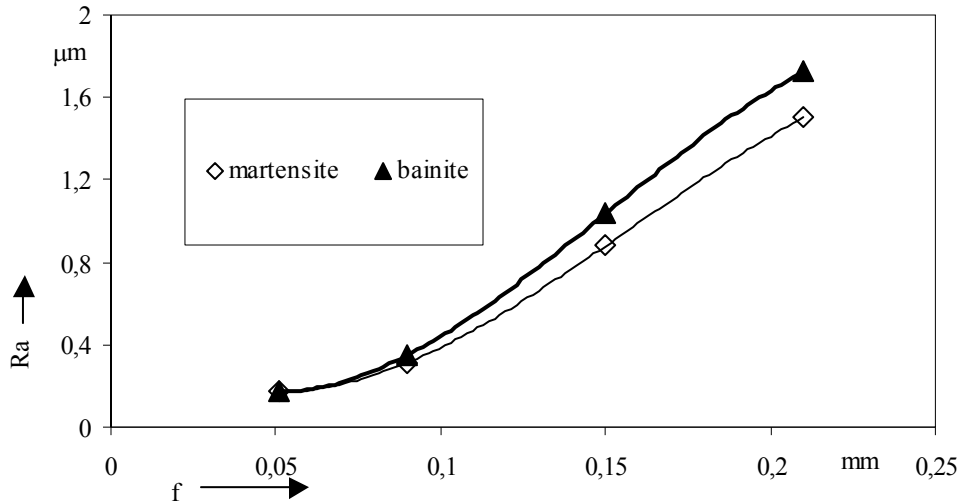
Fig.6 Influence of feed f on roughness of machined surface Ra
