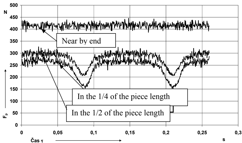
Fig.5 Record of cutting force F_p in the different places of the piece length 250 mm after bainite heat treatment (there is offset 100 N of F_p record for near by end of the piece)
