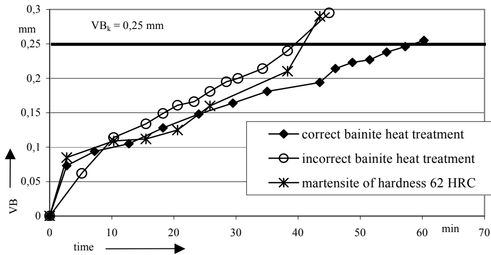
Fig.8 Process of tool wear, a_p = 0,25 \text{ mm} , f = 0,09 \text{ mm} , v_c = 85 \text{ mm} \cdot \text{min}^{-1}
