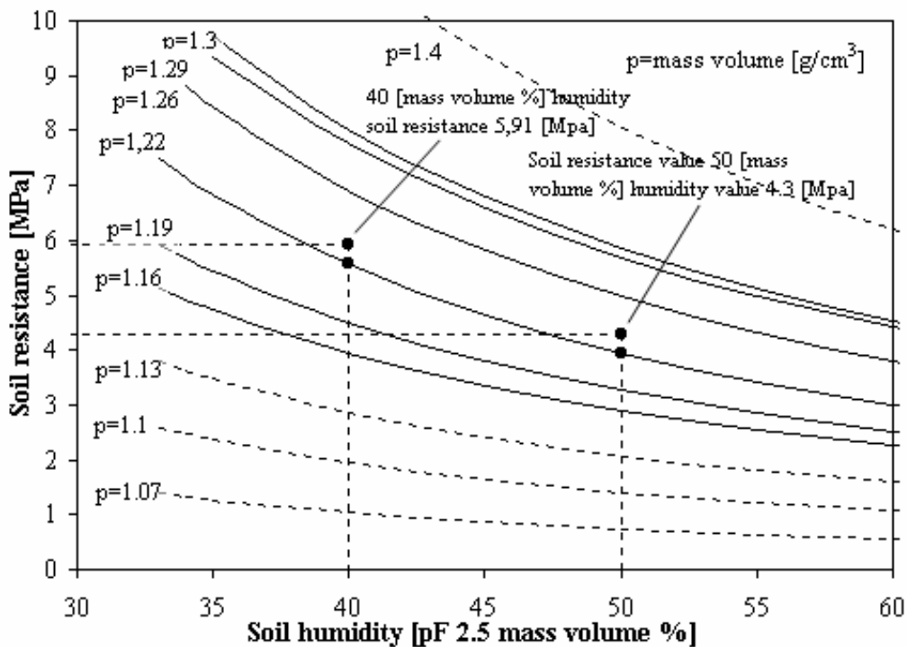
Fig. 1. The method of converting the soil resistance value at different humidity into identical soil humidity values
